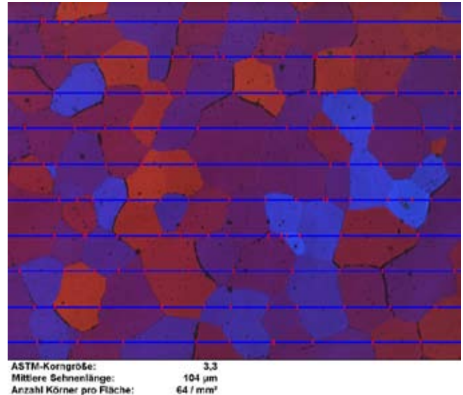
Figure 6. Grain size of a homogenized billet using ASTM standard
