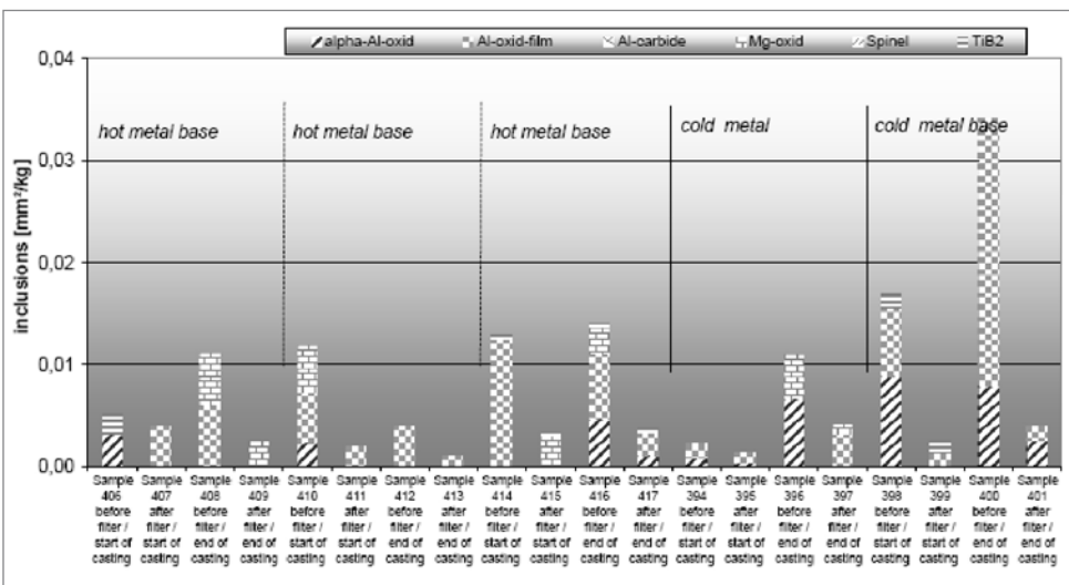
Figure 4. PodFa - measurements to compare inclusion amount using hot metal and cold metal (50%), before and after the ceramic foam filter-system accepted.
