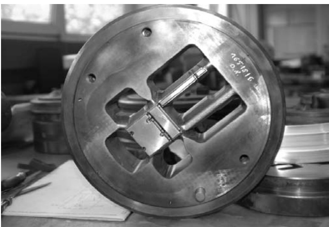
Figure 9. Tool for extruding gloss alloy
