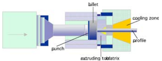
Figure 10. Extrusion process
