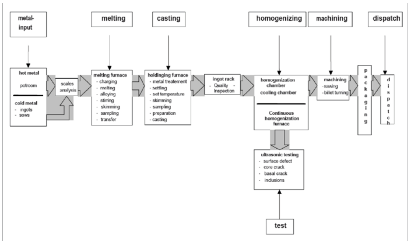
Figure 2. Production-flow cast house.
