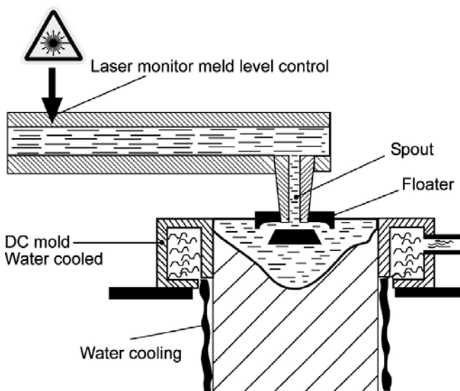
Figure 5. The casting system (3)
