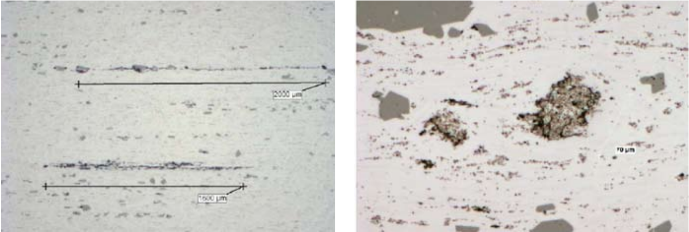
Figure 3. Unacceptable Oxide lines and TiB2 agglomerates in a grain refinement rod.
